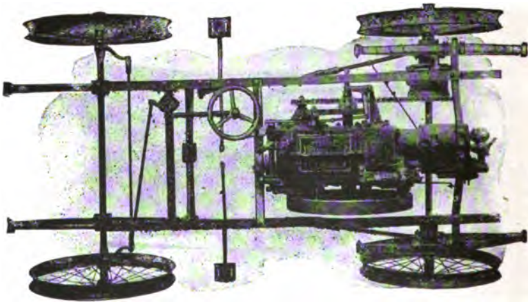
FIG. 408.—Plan View of the St. Louis Gasoline Carriage, showing motor and mechanism in position.
